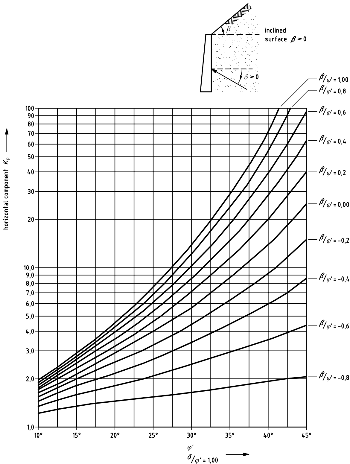
Figure C.2.4 — Coefficients K_p of effective passive earth pressure (horizontal component): with inclined retained surface ( \delta/\varphi' = 1 )
