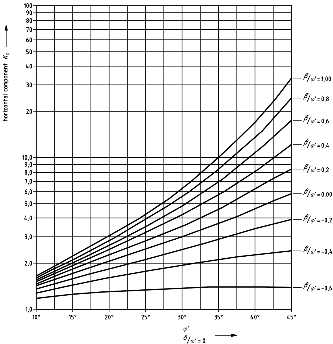
Figure C.2.2 — Coefficients K_p of effective passive earth pressure (horizontal component): with inclined retained surface ( \delta/\phi' = 0 and \delta = 0 )
