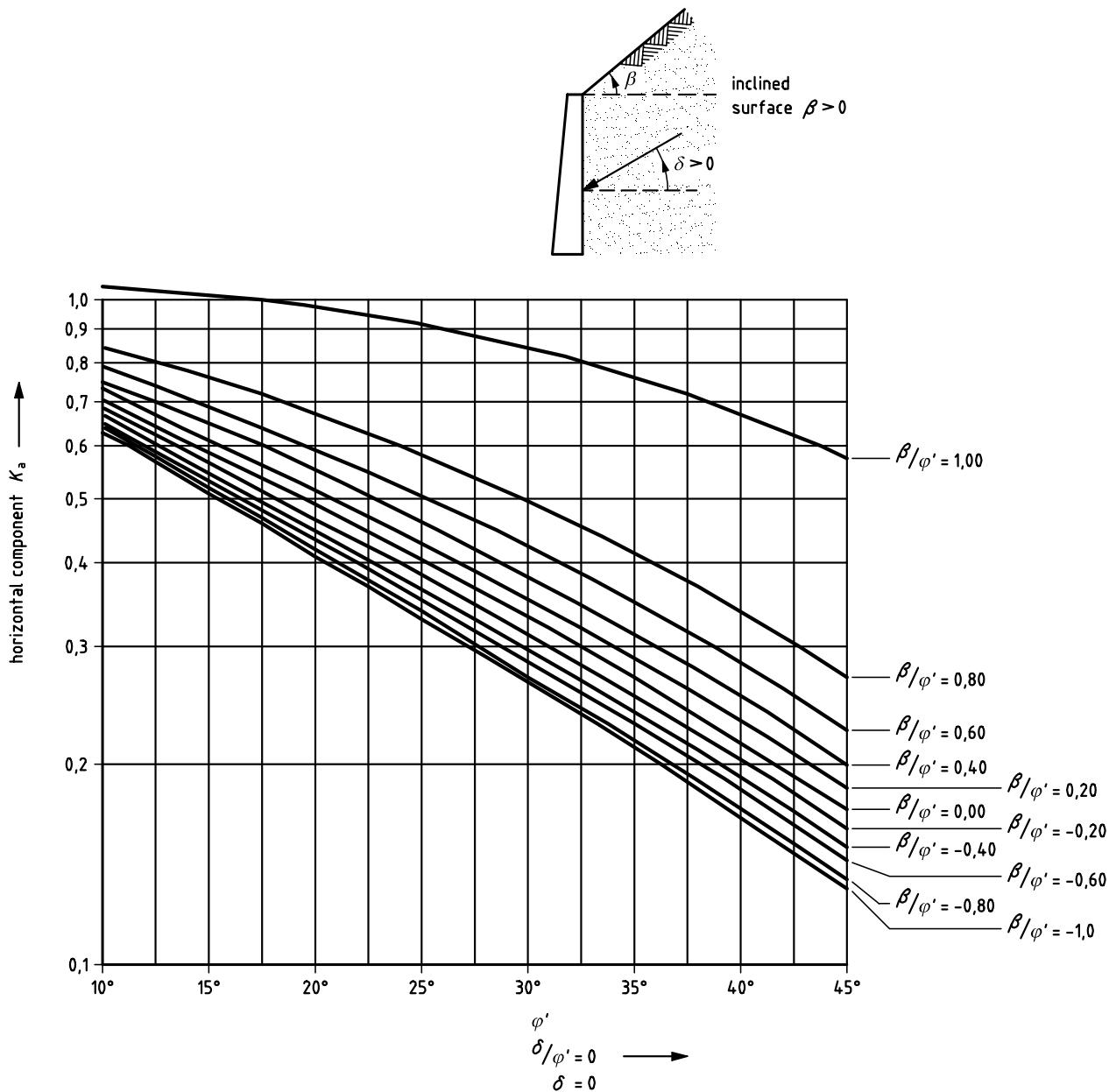
Figure C.1.2 — Coefficients K_a of effective active earth pressure (horizontal component): with inclined retained surface ( \delta/\varphi' = 0 and \delta = 0 )
