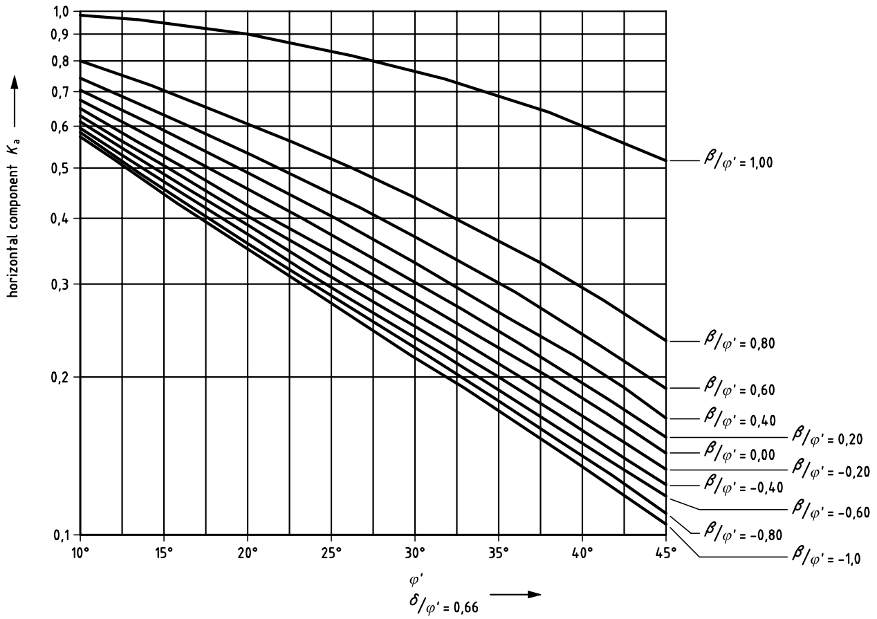
Figure C.1.3 — Coefficients K_a of effective active earth pressure (horizontal component): with inclined retained surface ( \delta/\varphi' = 0,66 )
