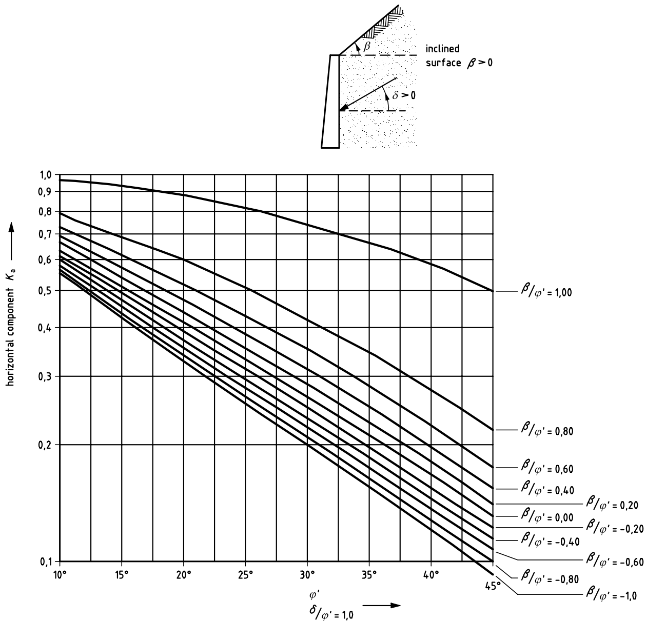
Figure C.1.4 — Coefficients K_a of effective active earth pressure (horizontal component): with inclined retained surface ( \delta/\varphi' = 1 )
