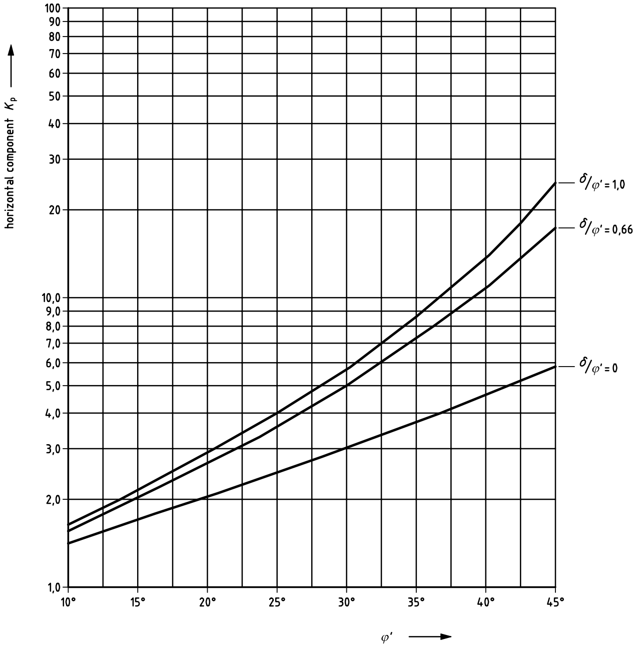
Figure C.2.1 — Coefficients K_p of effective passive earth pressure (horizontal component): with horizontal retained surface ( \beta = 0 )
