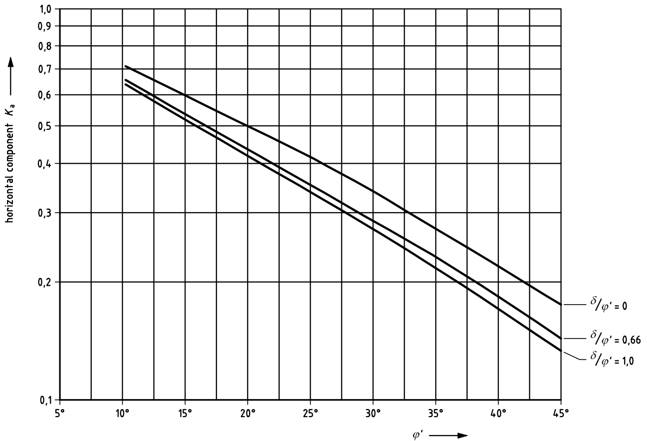
Figure C.1.1 — Coefficients K_a of effective active earth pressure (horizontal component): with horizontal retained surface ( \beta = 0 )
