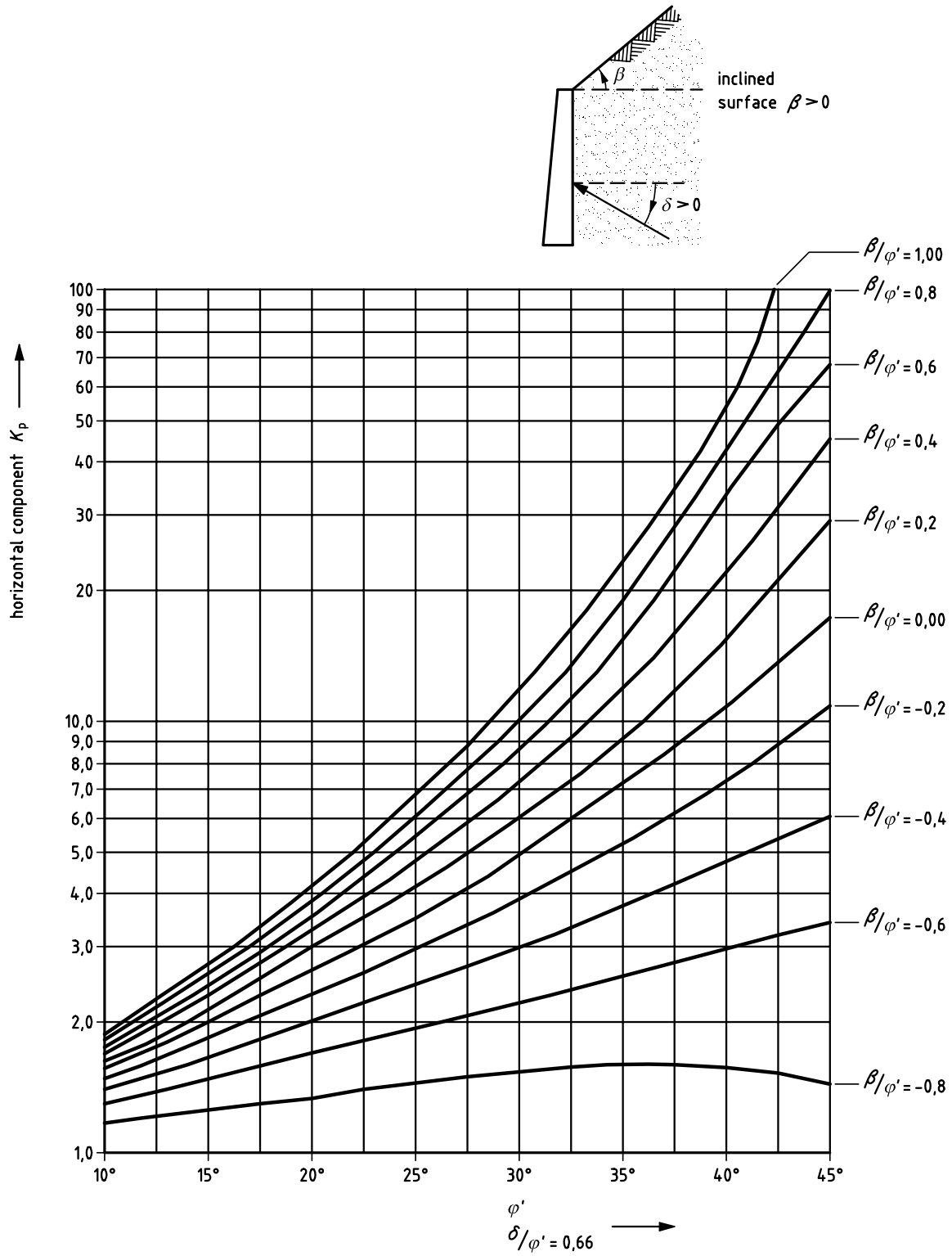
Figure C.2.3 — Coefficients K_p of effective passive earth pressure (horizontal component): with inclined retained surface ( \delta/\phi' = 0.66 )
